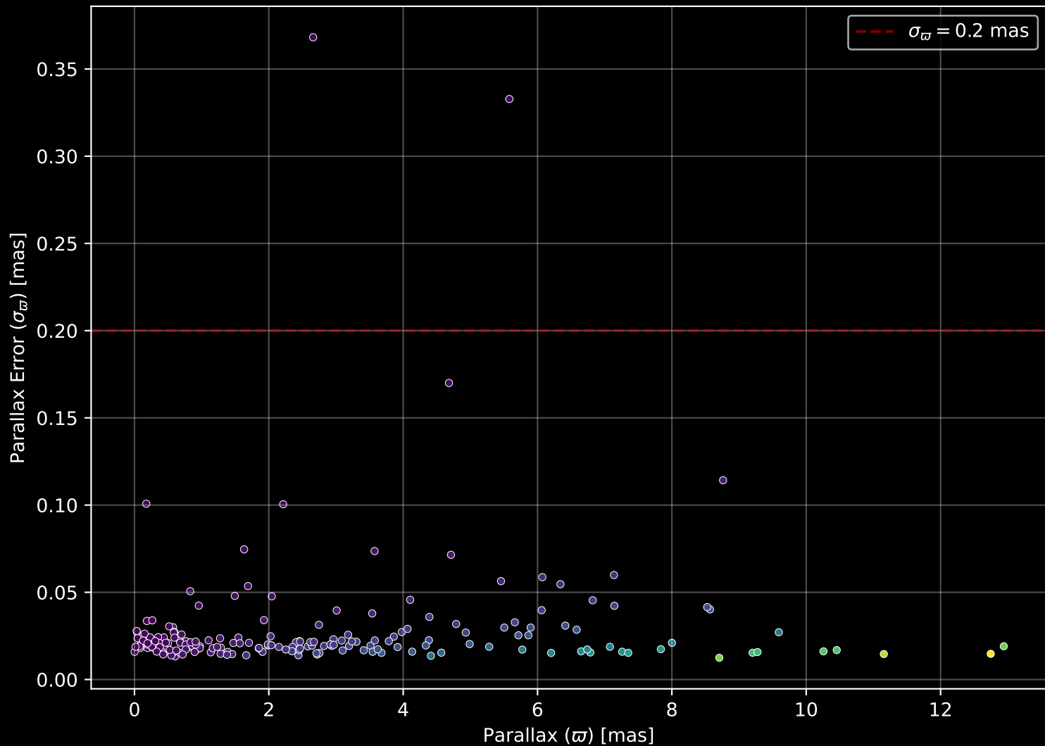
APOGEE DR17 Field: [250+60] Parallax Quality (n= 191)
