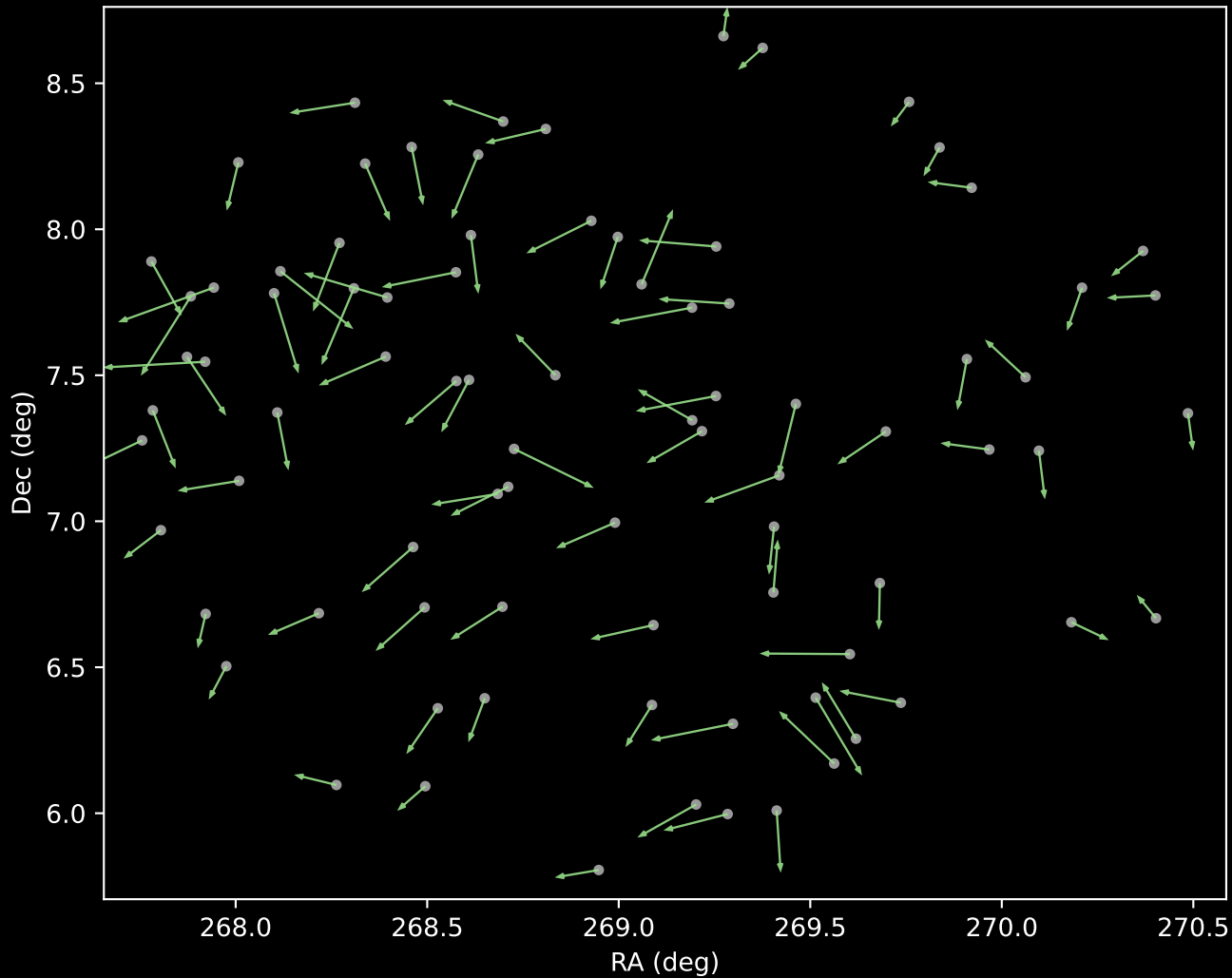
APOGEE DR17 Cluster 5 Proper Motion Vectors (n=84)
