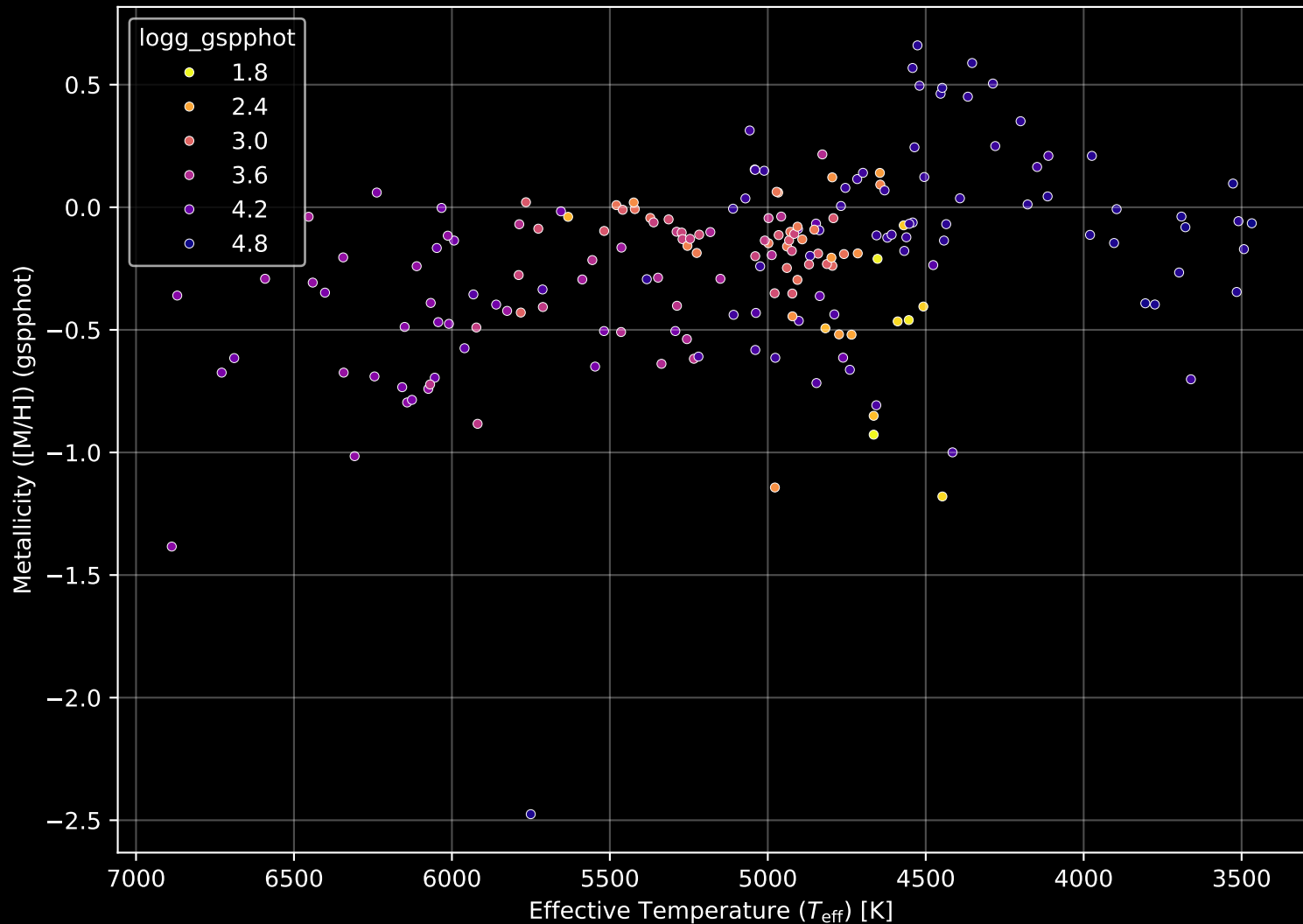
APOGEE DR17 Field: [250+60] Stellar Population Parameters (n= 191)
