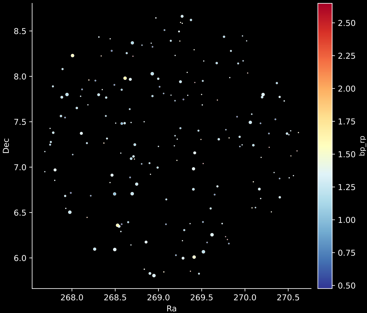
APOGEE DR17 Field: [250+60] Stars: 191
