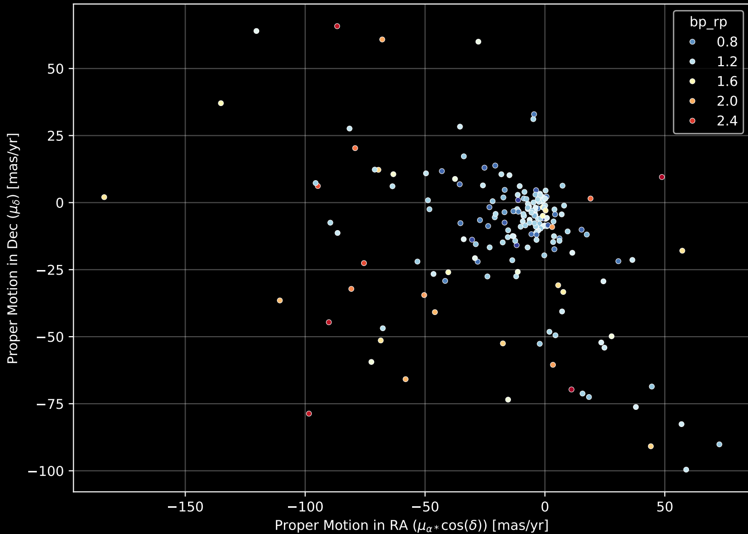
APOGEE DR17 Field: [250+60] Proper Motion Diagram (n= 191)
