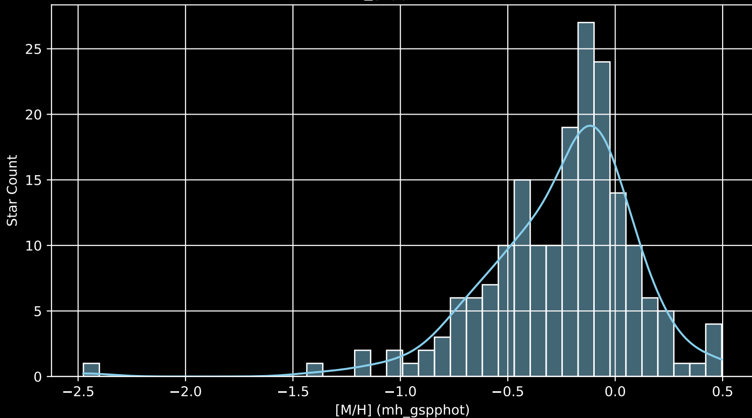
APOGEE DR17 Field: [250+60 [M/H] (mh_gspphot) (n= 187)
