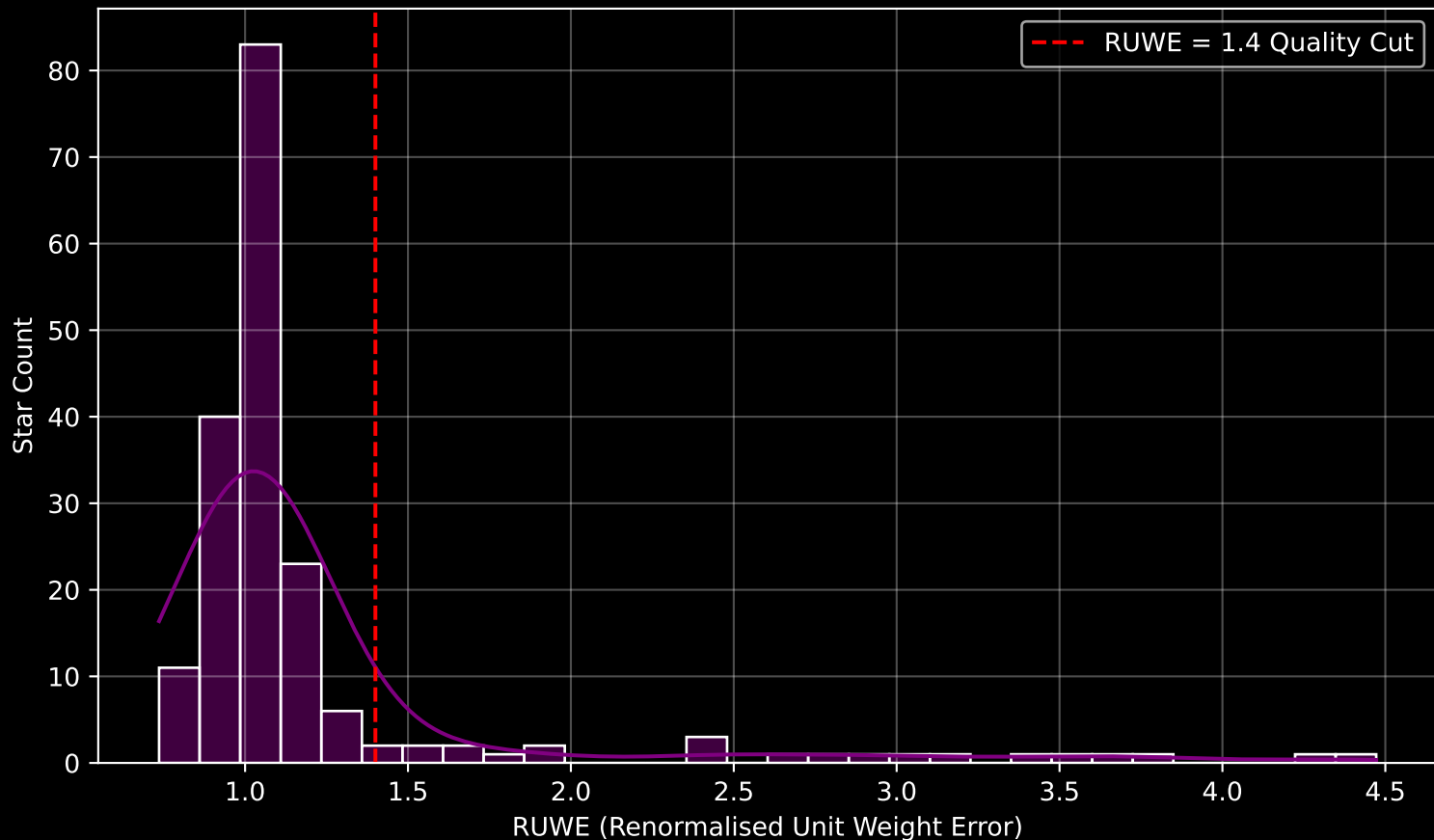
GAPOGEE DR17 Field [250+60] RUWE Distribution (n= 186)
