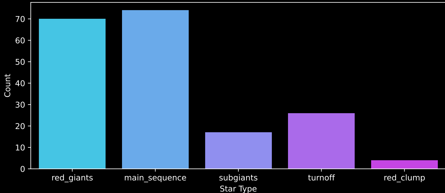
APOGEE DR17 Field: [250+60] Count plot of Star Type
